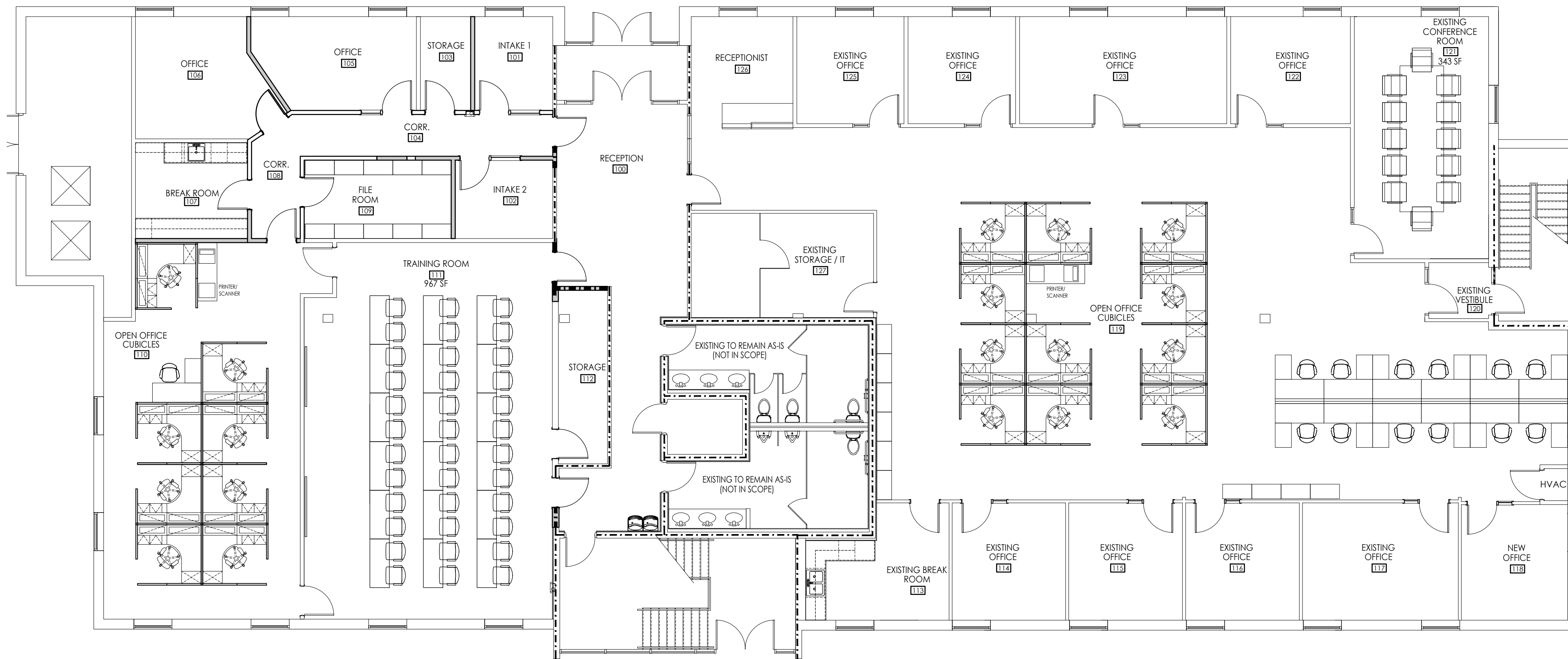
1 FURNITURE PLAN SCALE: 1/8"=1'-0"
